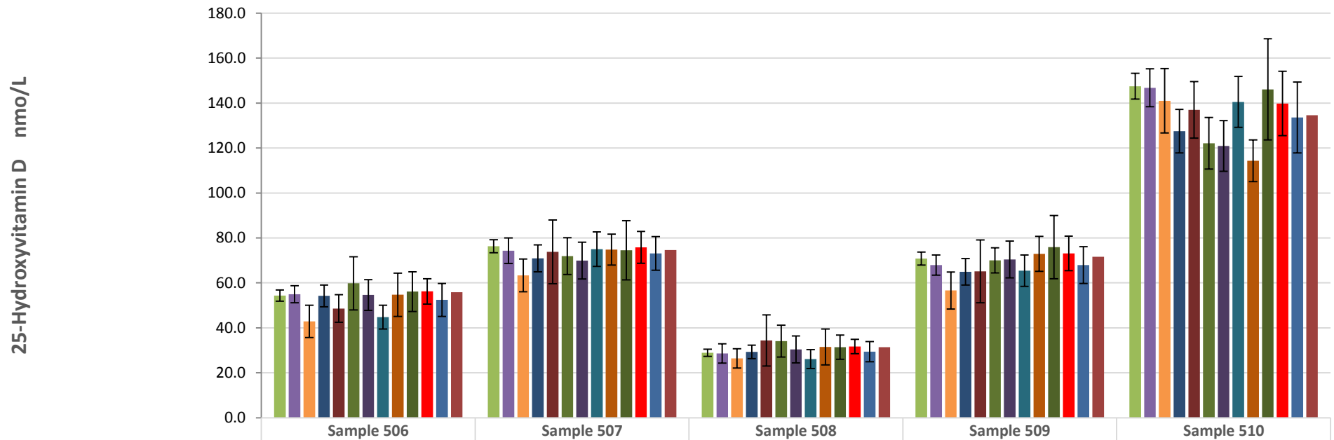
DEQAS January 2017 - 25-OHD Method Means (+/-1SD) for Major Method Groups*
